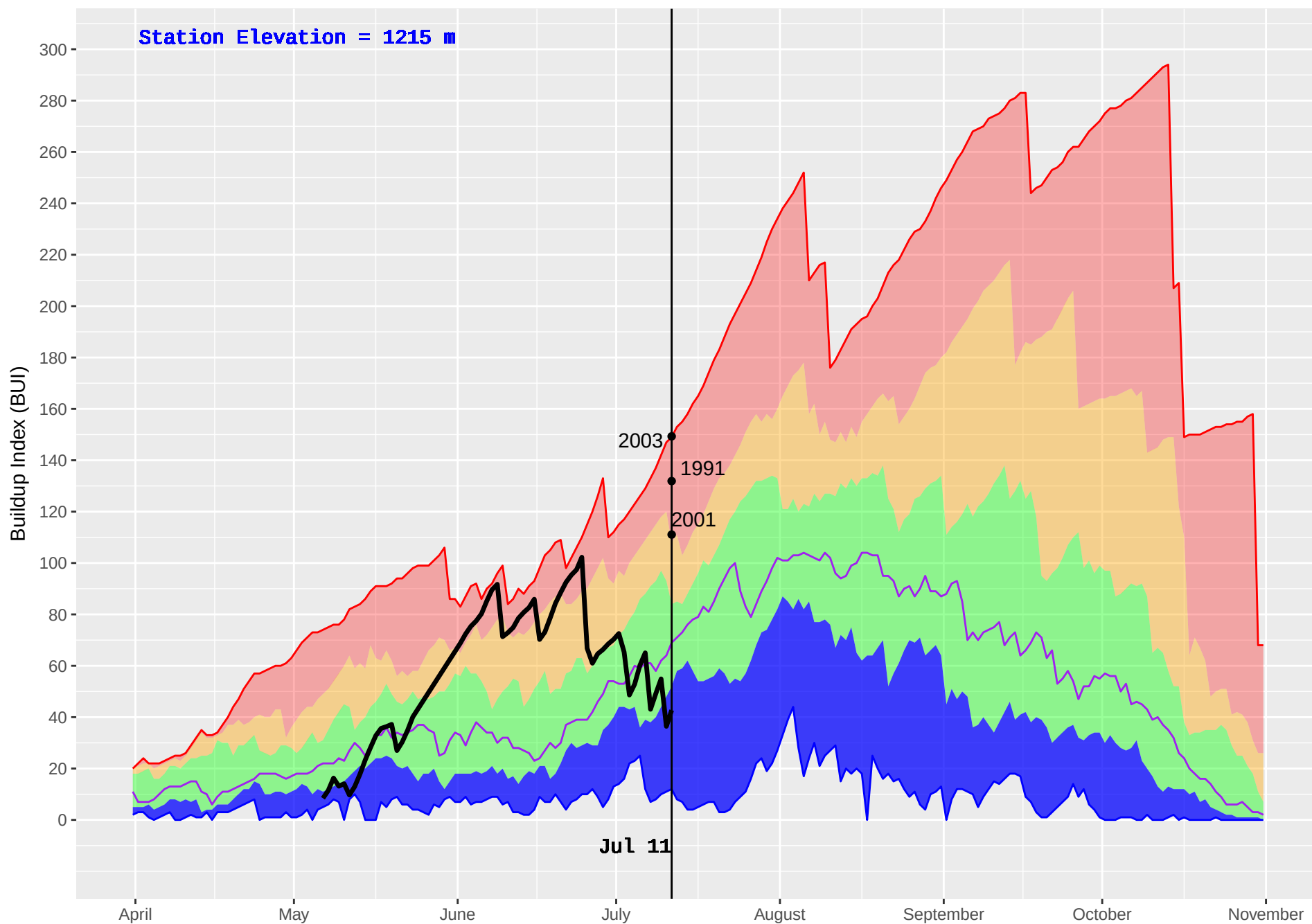
ALLISON PASS (317) : Historical (1987–2016) and Current (2018) Noon Buildup Index (BUI)
