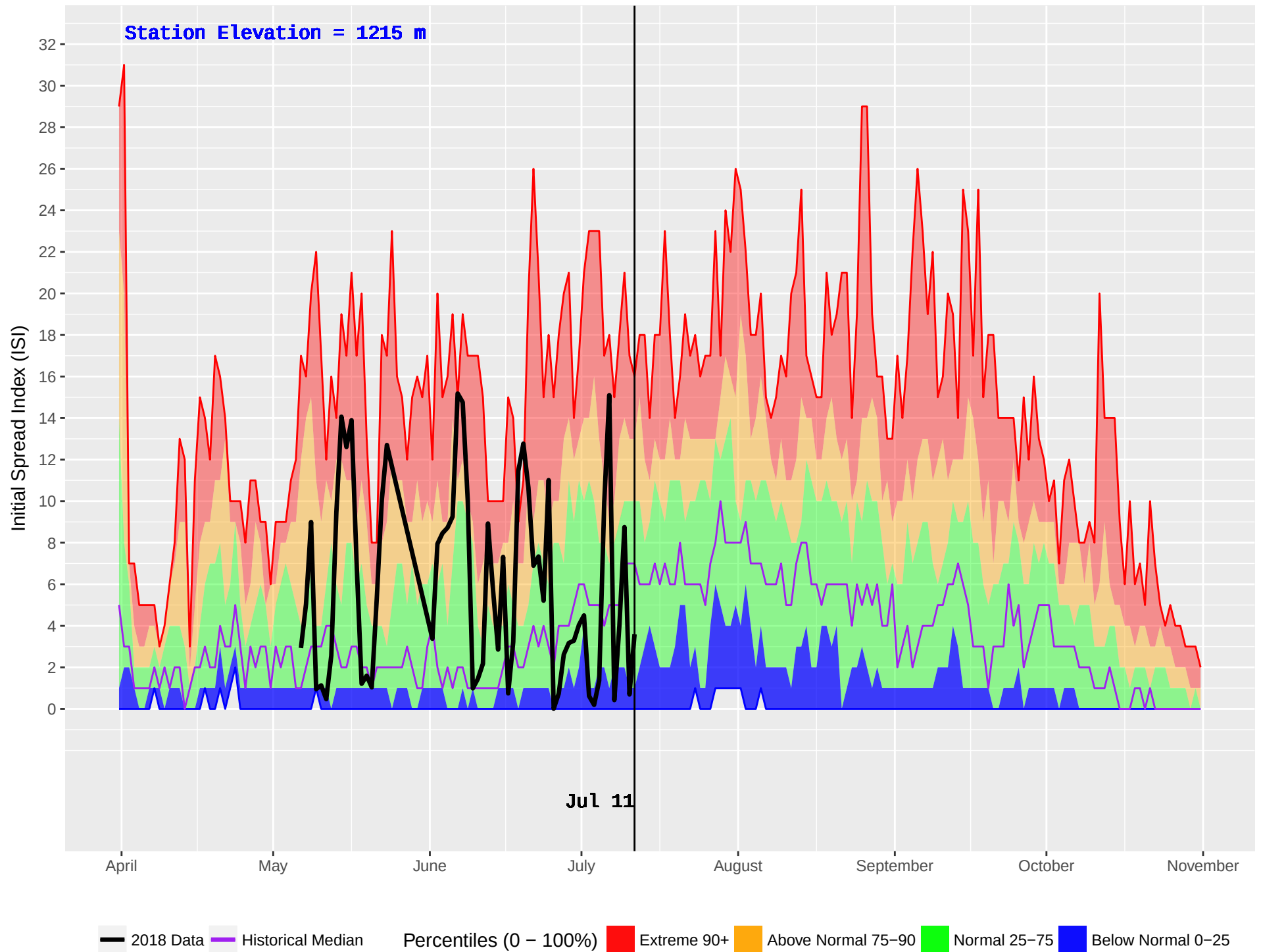
ALLISON PASS (317) : Historical (1987–2016) and Current (2018) Noon Initial Spread Index (ISI)
