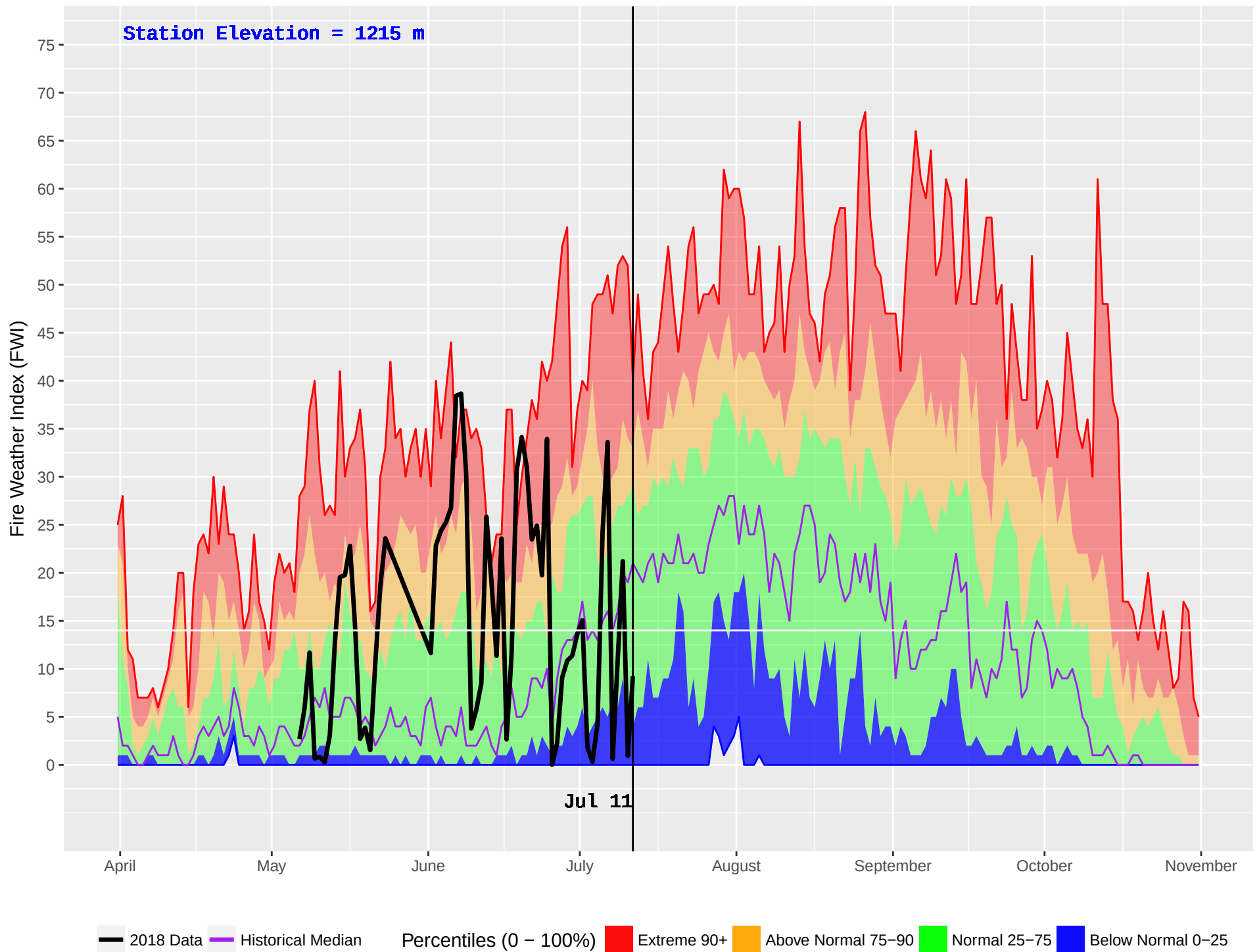
ALLISON PASS (317) : Historical (1987–2016) and Current (2018) Noon Fire Weather Index (FWI)
